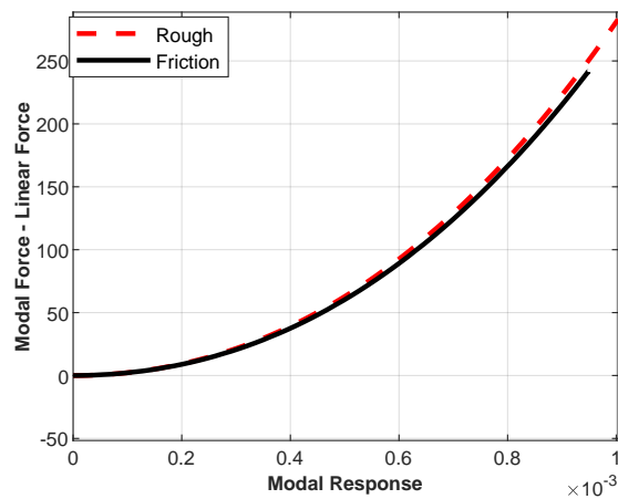
Figure 2: Load displacement curves for 2D TMD Benchmark model with an infinite coefficient of friction (i.e. “Rough” contact in Abaqus) and Lagrange friction with \mu = 0.6 .
