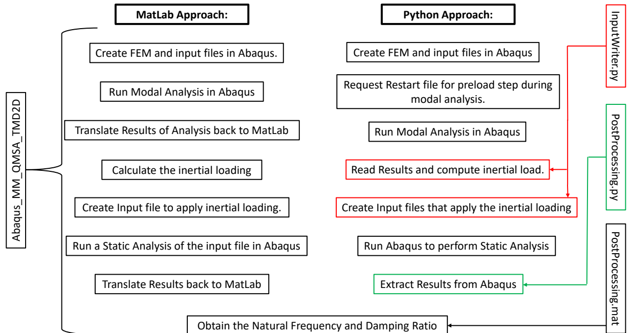
Figure 1: Flow chart representation of the two methods that are discussed in this work. The names of the scripts are given on the far sides of the flowchart, with Matlab on the left and Python on the right.
