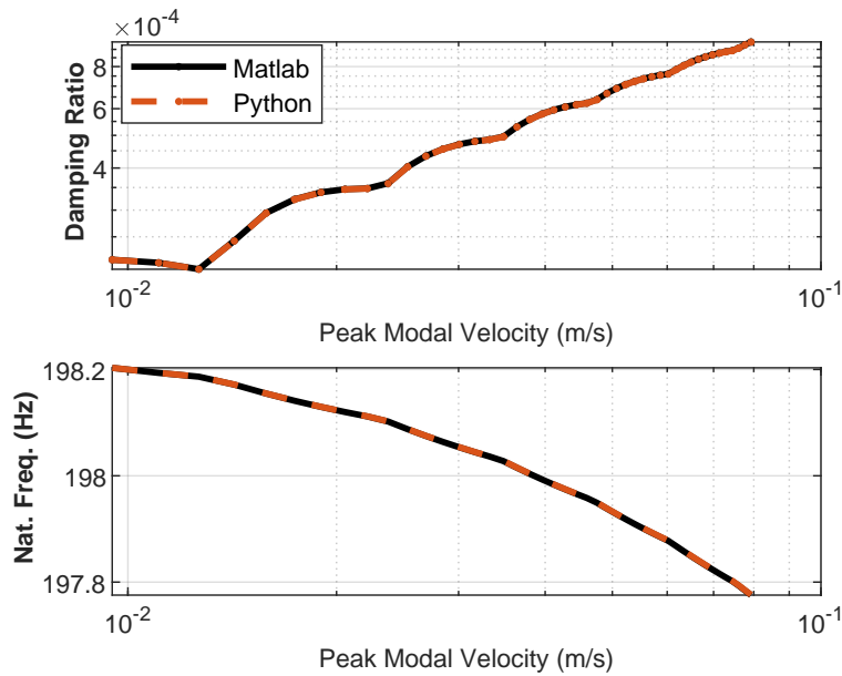
Figure 5: Comparison of the natural frequency and damping ratio obtained using the python scripts that are described in this work and the previous Matlab script for the Stacked Beam model. The results differ only in the 3rd decimal place.
