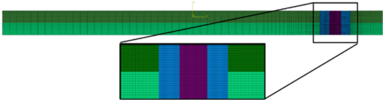
Figure 3: Visual representation of the Stacked Beam model that is used in Section 3. The magnified portion of the Figure represents the pressure load that is implemented to represent a bolt that holds the two plates together.
