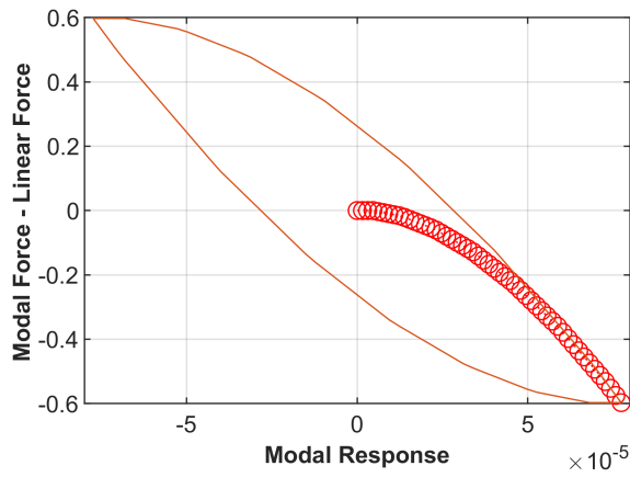
Figure 4: Example of a modal force-displacement result for the 2D Beam, as well as the resulting hysteresis loop that is formed by using Masing's rules. As is mentioned in [8], the slope of the secant line of the force-displacement backbone is used to calculate the natural frequency of the system, and the area enclosed in the hysteresis loop is used to find the damping ratio of the system.
