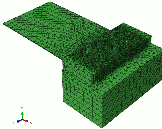
Figure 7: 3D FE model of the support, blades and panel, dubbed here the partial assembly because half-symmetry was employed.
