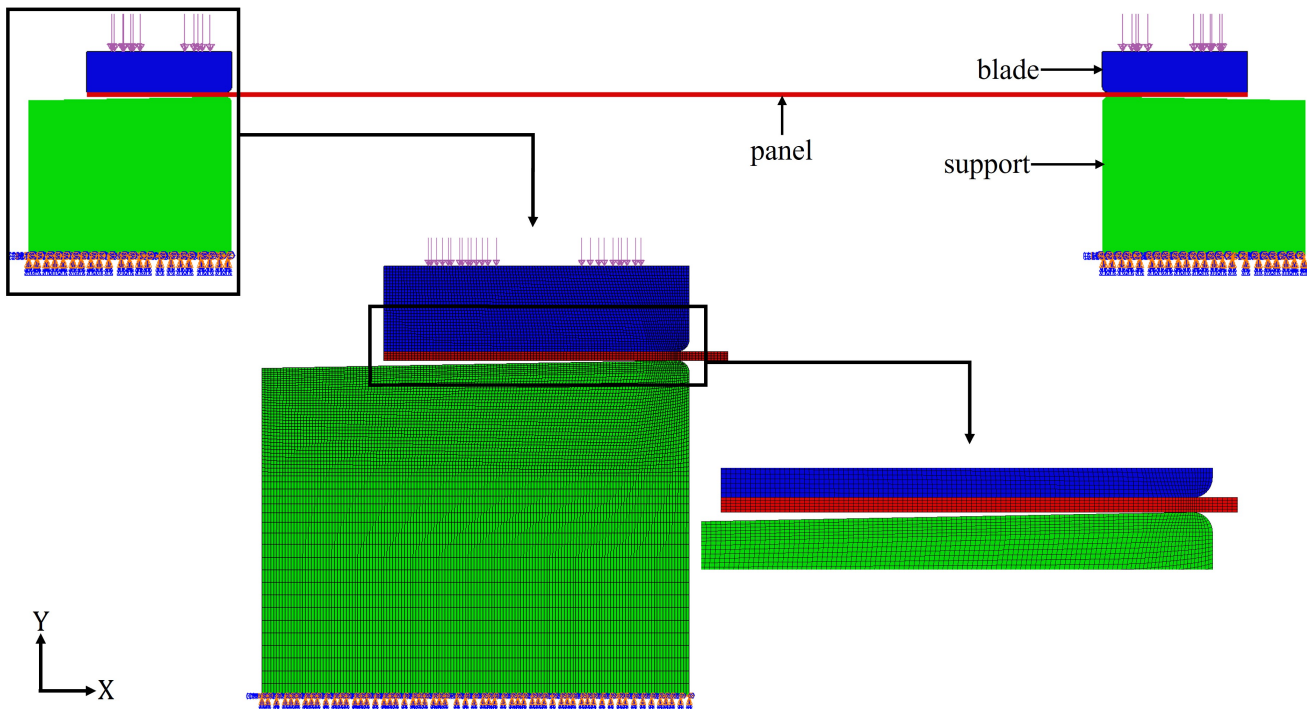
Figure 6: 2D FE model of the TMD structure, with a magnified version of the left-hand side interface showing the mesh density at contact, from [14].
