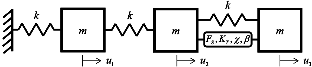
Fig. 3. Schematic of the three-mass system with a discrete Iwan joint model connecting the second and third masses.
