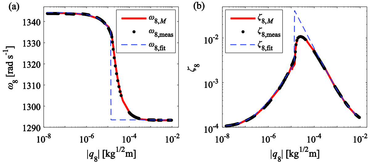
Fig. 11. (a) Natural frequency and (b) critical damping ratio versus modal displacement for selective excitation of mode 8 of the Sumali beam.
