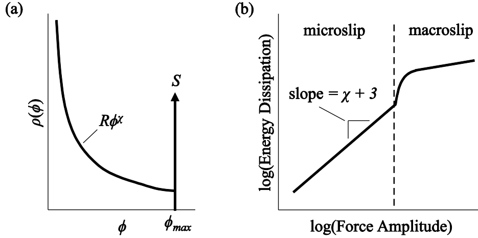
Fig. A.2. (a) The population distribution function of slider strengths associated with the four-parameter Iwan model, and (b) the resulting log-log energy dissipation per cycle for that model.
