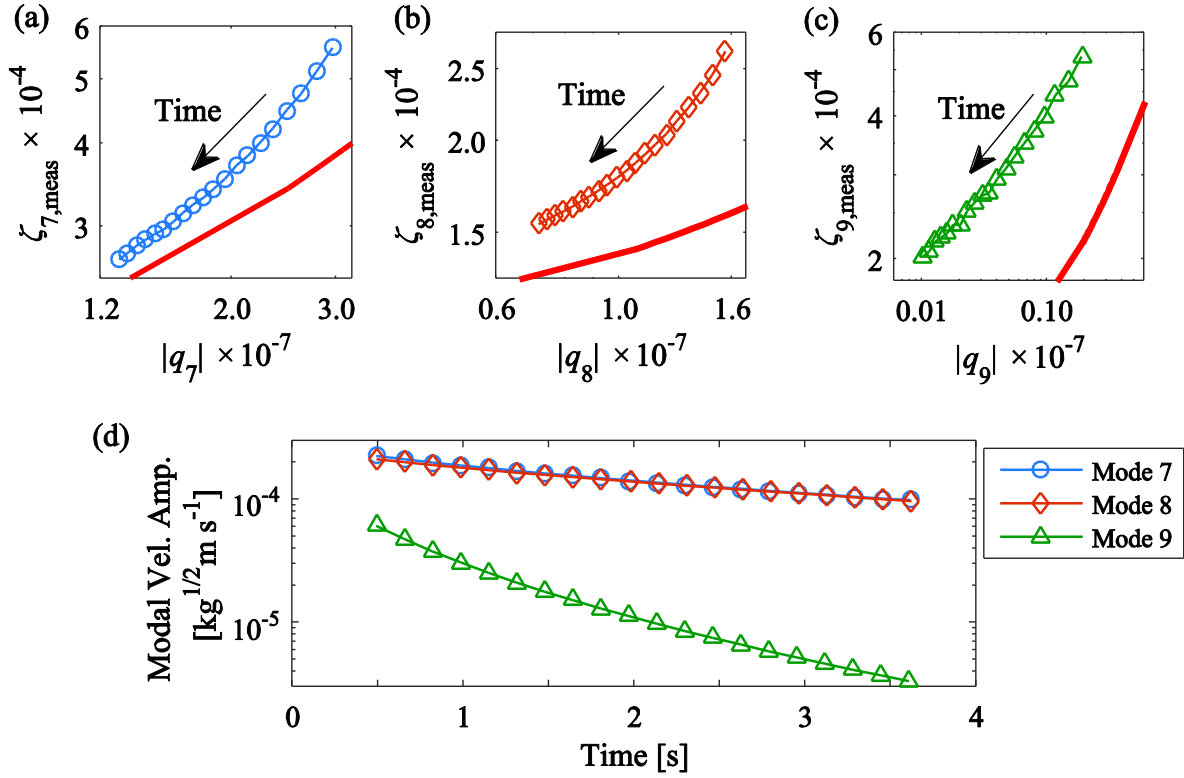
Fig. 15. Damping versus displacement amplitude with ideal curves in (a) mode 7, (b) mode 8, and (c) mode 9 response to an impulse in the Sumali beam (shown with \zeta_{r,M} as the thick curve), and (d) time histories of the velocity amplitude for the three modes. The data are from simulation 6 in Table D.2. Displacement amplitude units are \text{kg}^{1/2} \text{m} .
